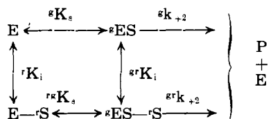
FIG. 2.—There are n possible complexes of the type {}^s\text{ES} , q of the type \text{E} \text{---} \text{}^r\text{S} , and nq of the type {}^s\text{ES} \text{---} \text{}^r\text{S} . There are n constants of the type {}^sK_s and {}^s k_{+2} , q of the type {}^rK_i , and nq of the types {}^rK_s , {}^{sr}K_i and {}^{sr}k_{+2} .
